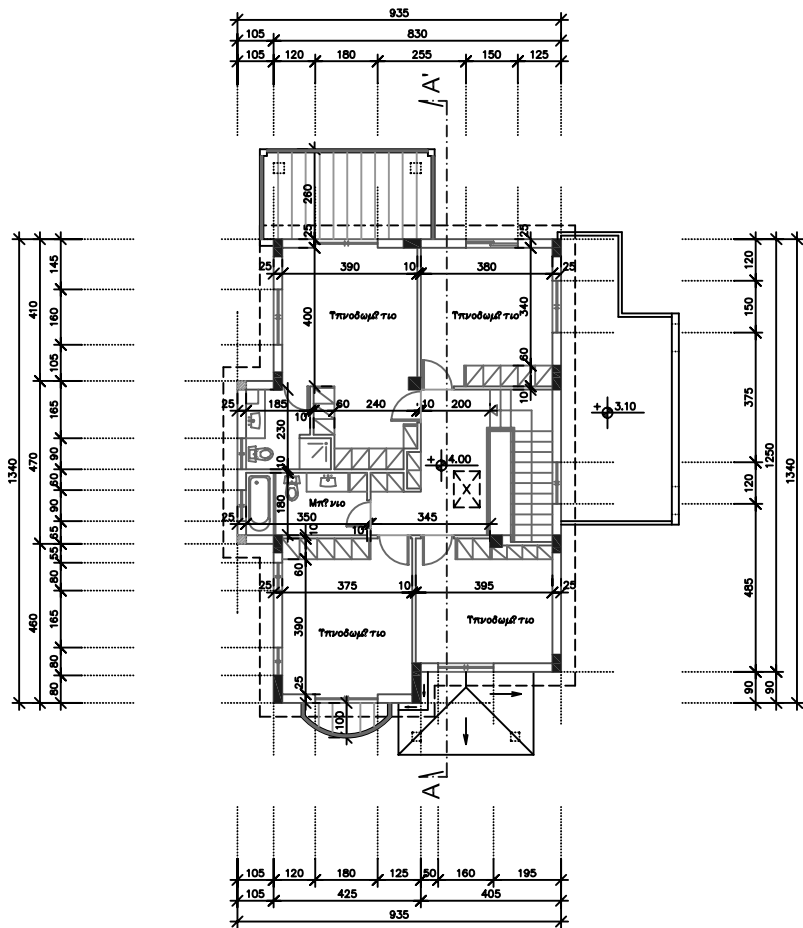
ΚΑΤΟΨΗ ΟΡΟΦΟΥ / Second Floor Plan
